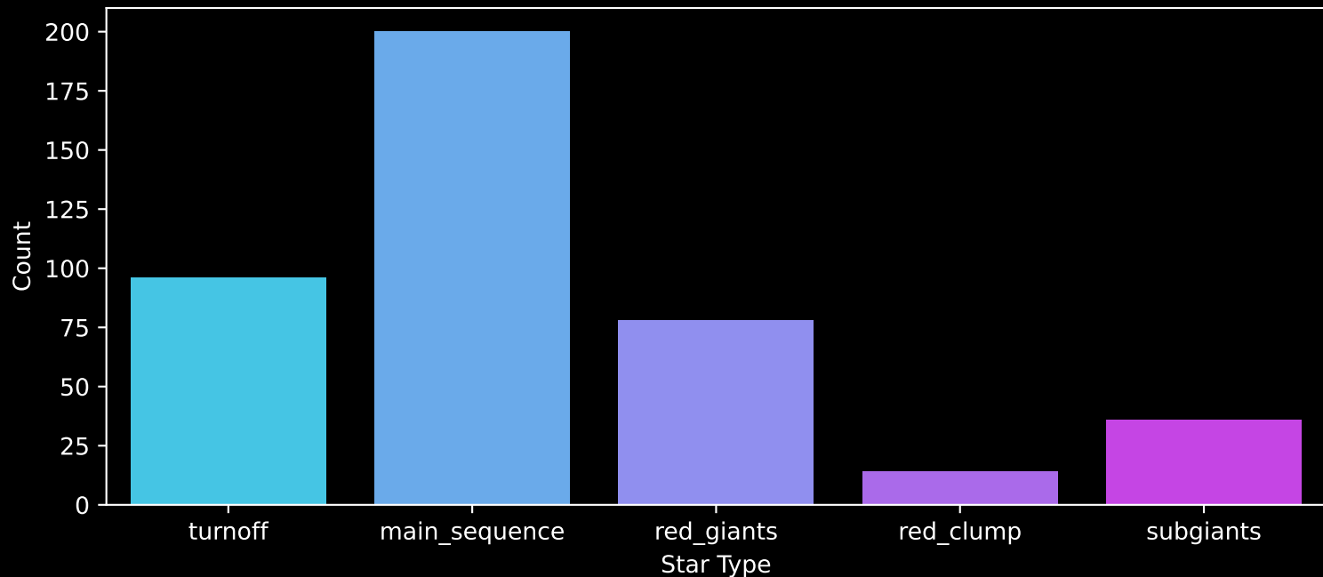
GALAH DR4 Field: [6591] Count plot of Star Type
