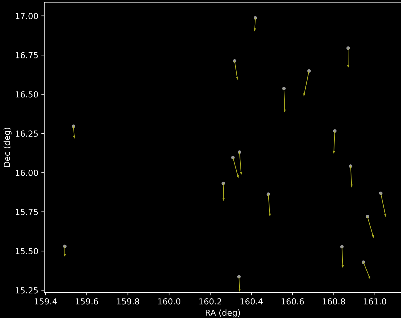
GALAH DR4 Cluster 16 Proper Motion Vectors (n=18)
