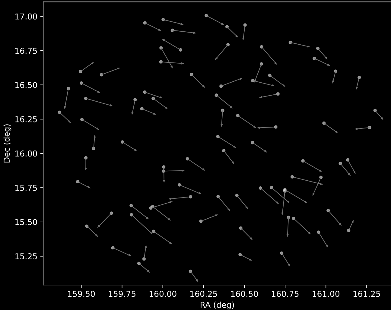
GALAH DR4 Cluster 14 Proper Motion Vectors (n=83)
