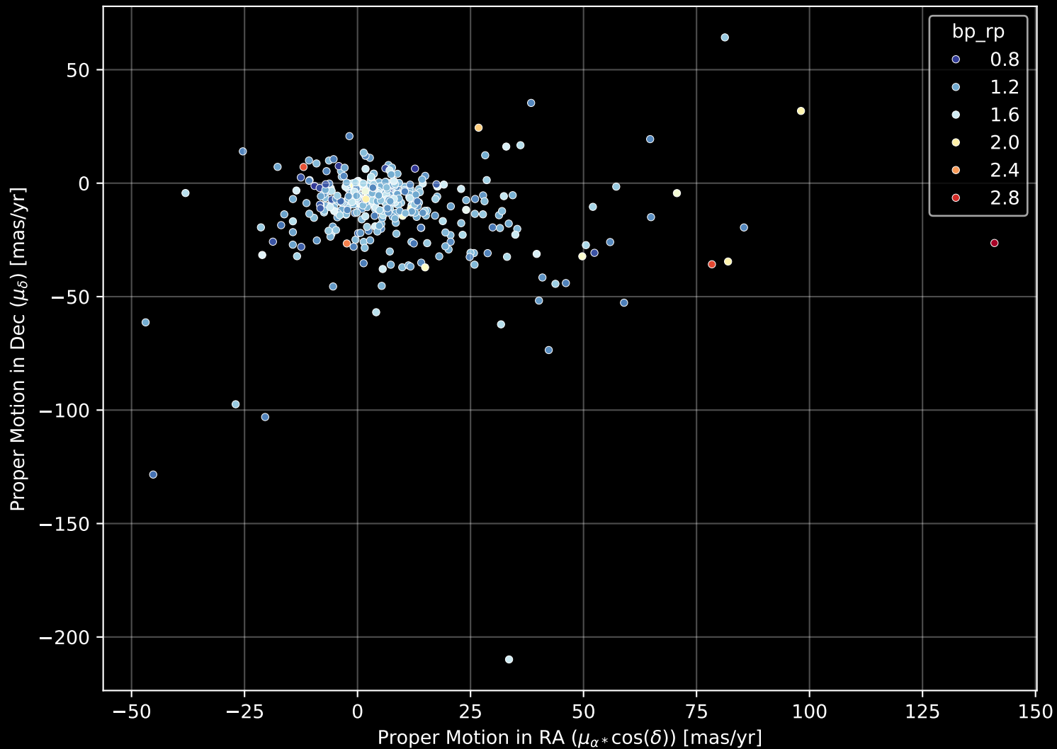
GALAH DR4 Field: [6591] Proper Motion Diagram (n= 424)
