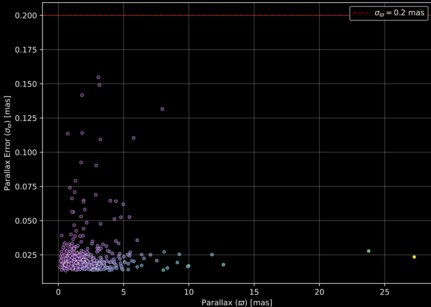
GALAH DR4 Field: [6591] Parallax Quality (n= 424)
