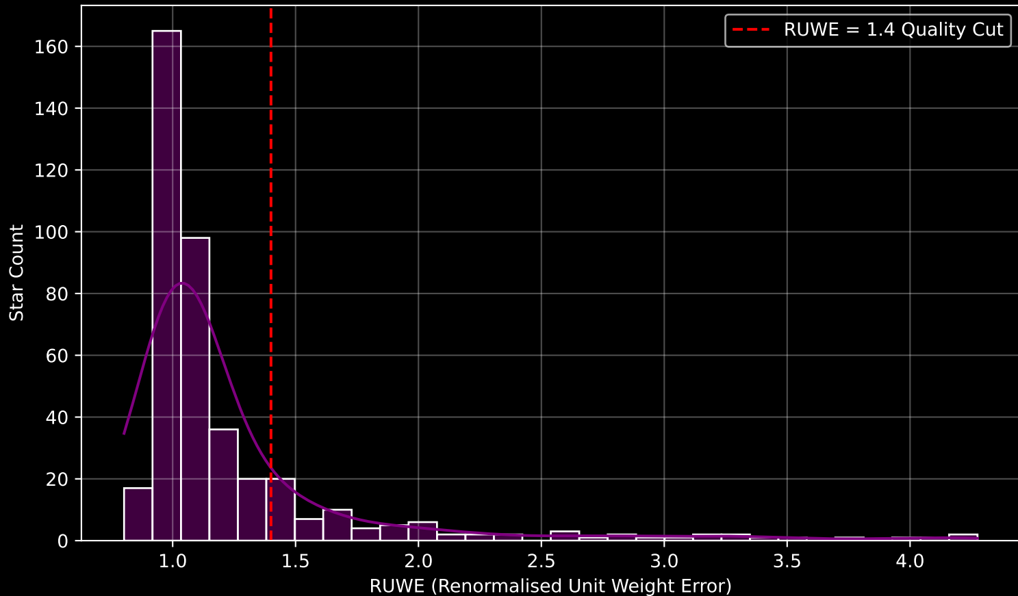
GALAH DR4 Field [6591] RUWE Distribution (n= 413)
