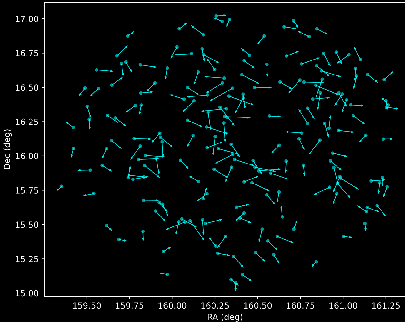
GALAH DR4 Noise Stream Proper Motion Vectors (n=189)
