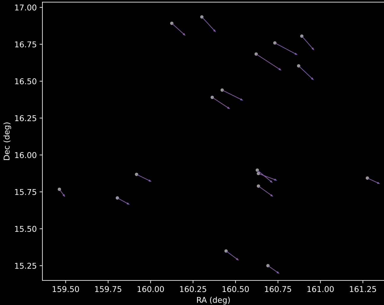
GALAH DR4 Cluster 8 Proper Motion Vectors (n=17)
